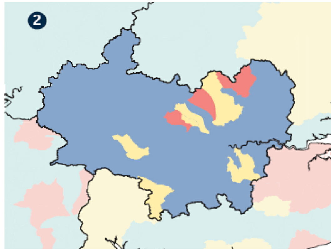
2. Winter surface water
