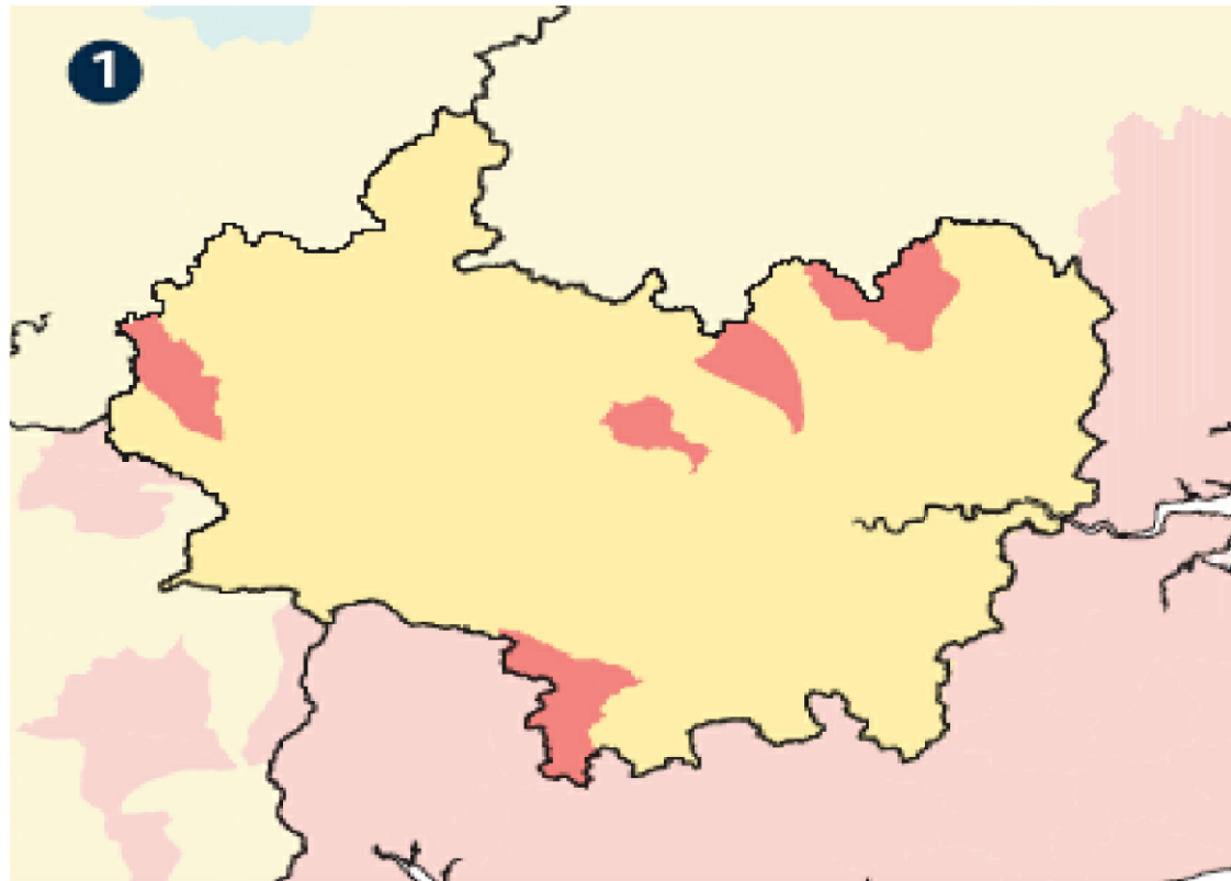
1. Summer surface water
