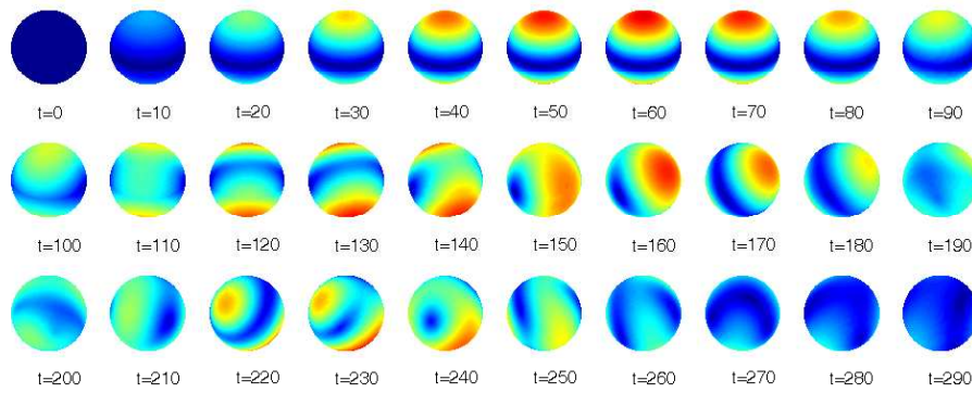
Fig. 8 (Color online) Snapshot sequence of the dynamic field u representing the transient evolution of the parse in Fock space.
