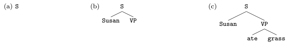
Fig. 2 Left-derivation (3) of the sentence Susan ate grass according to grammar (1).
