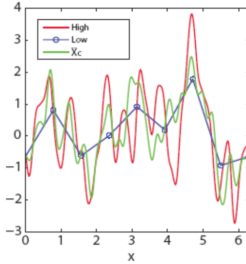
Figure 6. Example high-resolution state, low-resolution state ( M = 8 ), and mean of the conversion density, which is labeled above as the “best estimate”. The low-resolution state is defined only at the grid-points denoted by the open circles.
