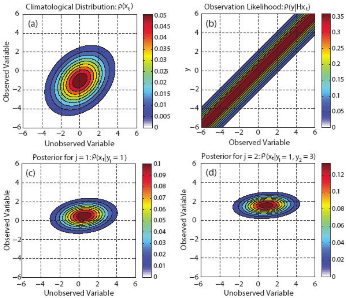
Figure 1. Data assimilation on the high-resolution (true) attractor. (a) High-resolution climatological distribution, (b) high-resolution observation likelihood, (c) high-resolution posterior for j = 1 , and (d) high-resolution posterior for j = 2 .
