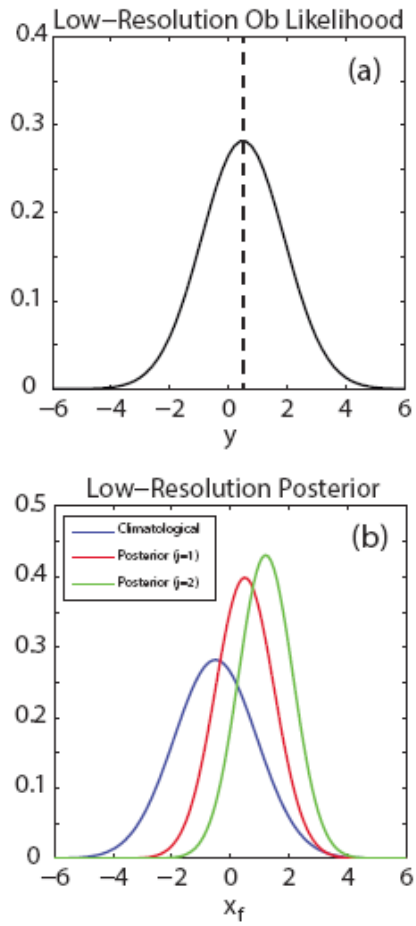
Figure 4. Data assimilation on the low-resolution (forecast) attractor. The low-resolution a) observation likelihood and b) climatological and posterior distributions for j = 1 and 2.
