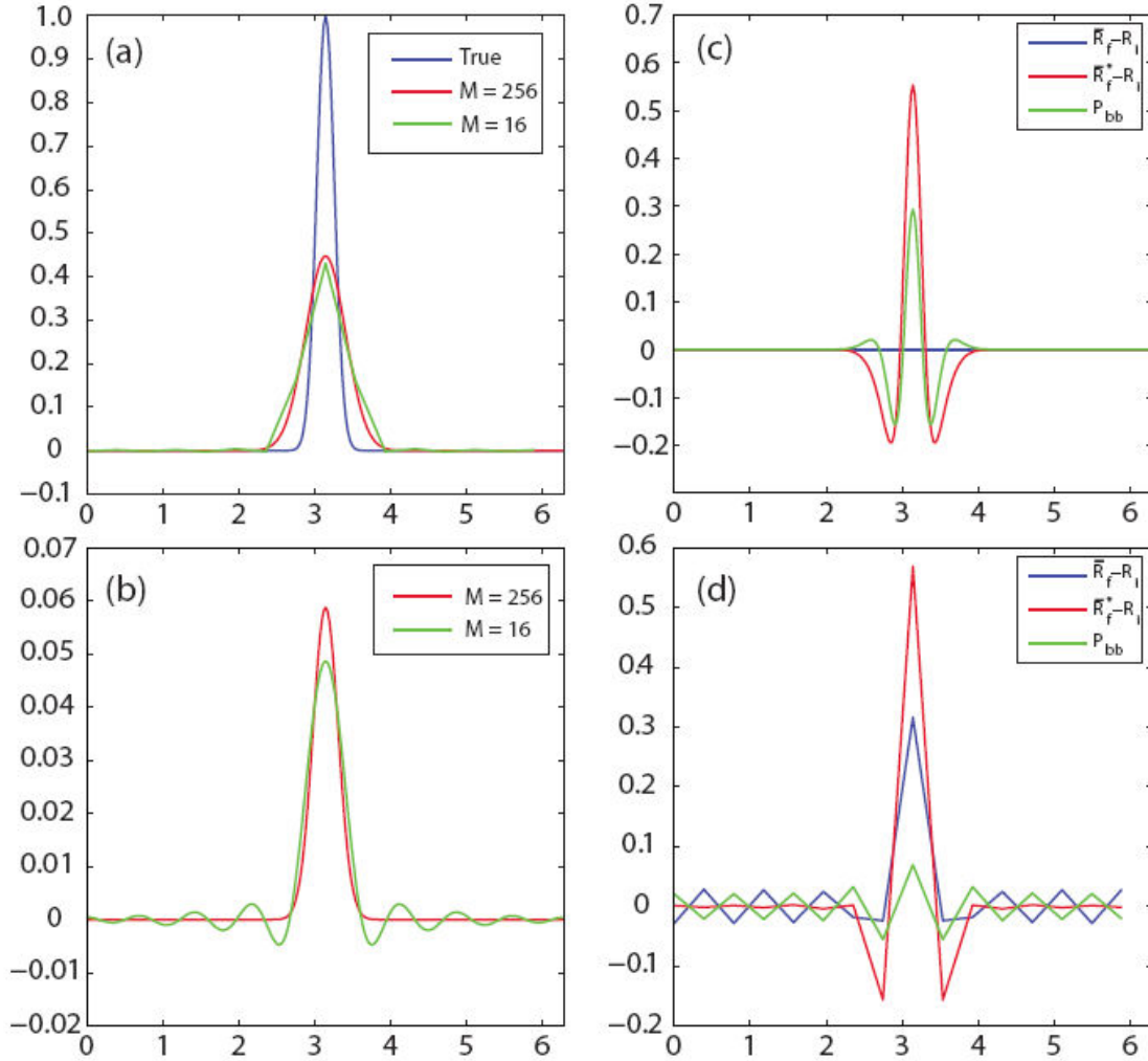
Figure 7. Gaussian Smoothing. In (a) are three one-point prior covariance functions: blue is the high-resolution (true) covariance model, red is the M = 256 low-resolution (forecast) covariance model, green is the M = 16 low-resolution (forecast) covariance model. In (b) are one column of the smoother matrix for M = 256 (red) and M = 16 (green). In (c) and (d) is shown the main components of the theory for M = 256 and M = 16 , respectively: blue is the representation error covariance ( \bar{\mathbf{R}}_f - \mathbf{R}_i ), red is the effective representation error covariance ( \bar{\mathbf{R}}_f^* - \mathbf{R}_i ), and green is the bias covariance matrix ( \mathbf{P}_{bb} ).
