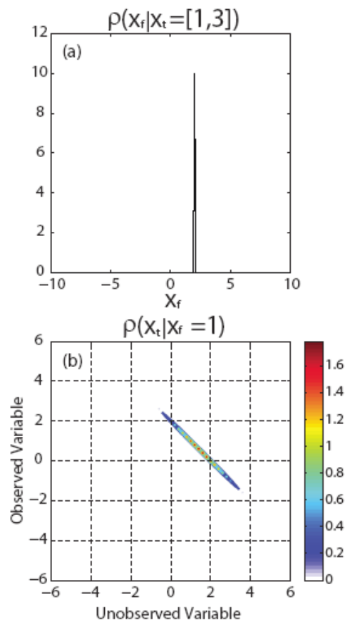
Figure 3. The conversion densities. In (a) is the conversion density describing the distribution of forecast states given a state on the true attractor ( x_t = [1 \ 3]^T ) and in (b) is the conversion density describing the distribution of true states given a state on the forecast attractor ( x_f = 1 ).
