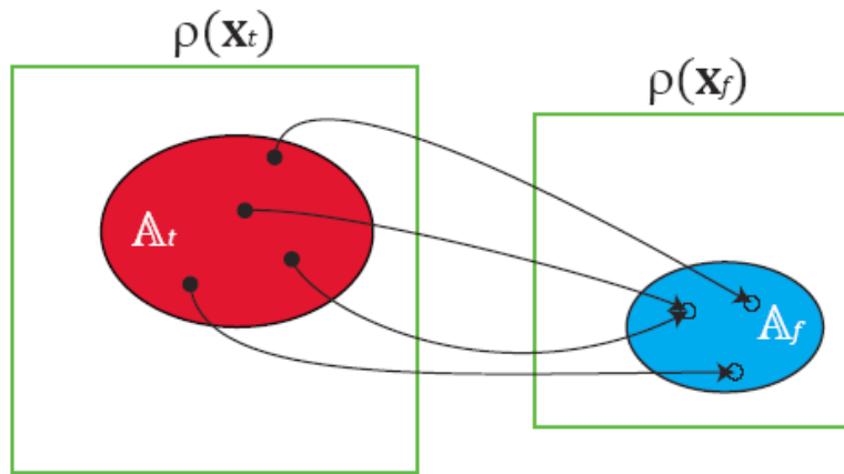
Figure 2. The attractors and their map. The two green squares represent the domain of the true states (large square) and the forecast states (small square). The region for which \rho(\mathbf{x}_t) > 0 ( \rho(\mathbf{x}_f) > 0 ) is denoted as the red (blue) shaded region. An example of the function in equation (2.3) is denoted by the arrows, which travel from states in \mathbb{A}_t denoted by filled circles to states in \mathbb{A}_f denoted by open circles. Note that multiple states in \mathbb{A}_t may map to the same point in \mathbb{A}_f . We will show that this results in an error of representation.
